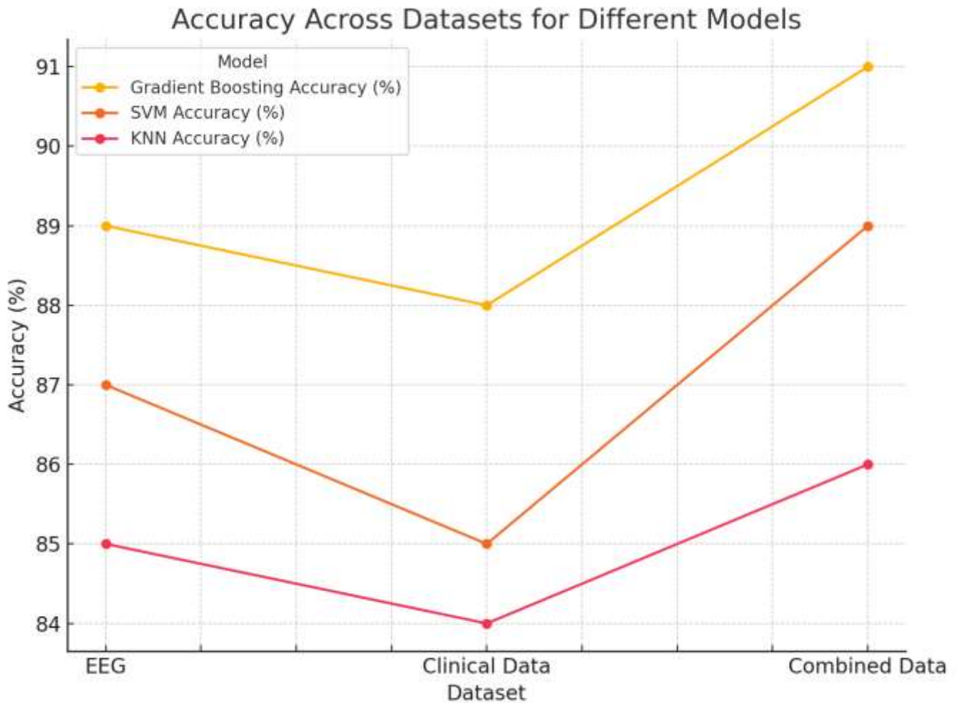
Figure 5: Accuracy across datasets for different models
