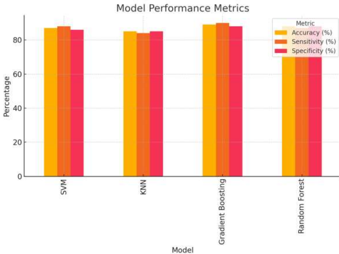
Figure 4: Model performance metrics
