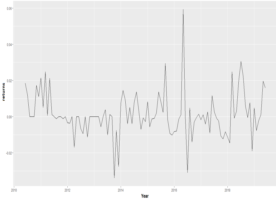
Figure 1: Time series plot of the monthly DZAIINDEX training returns
