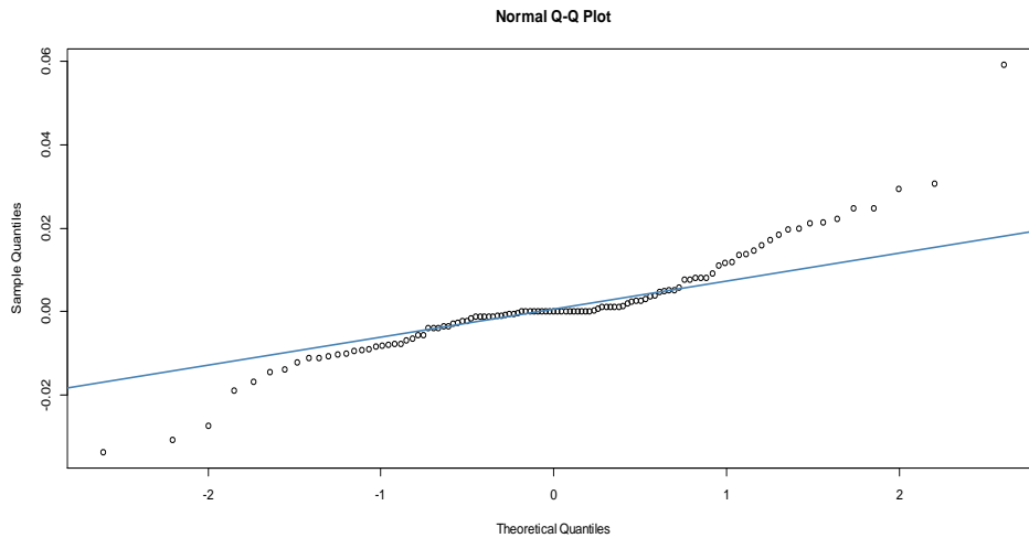
Figure 2: Q-Q Plot of the monthly DZAIINDEX training returns time series
